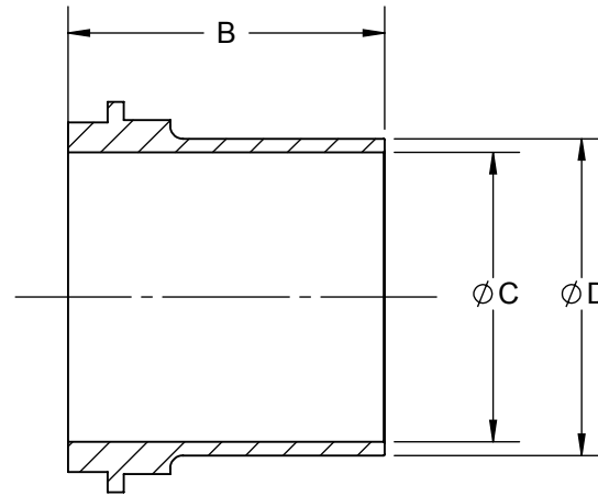
SECTION X-X
